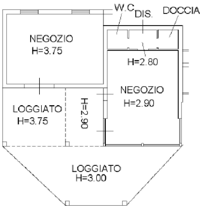
PIANO TERRA
