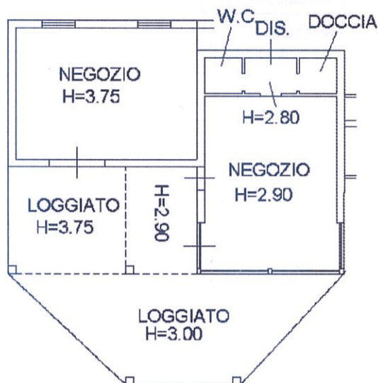
PIANO TERRA
