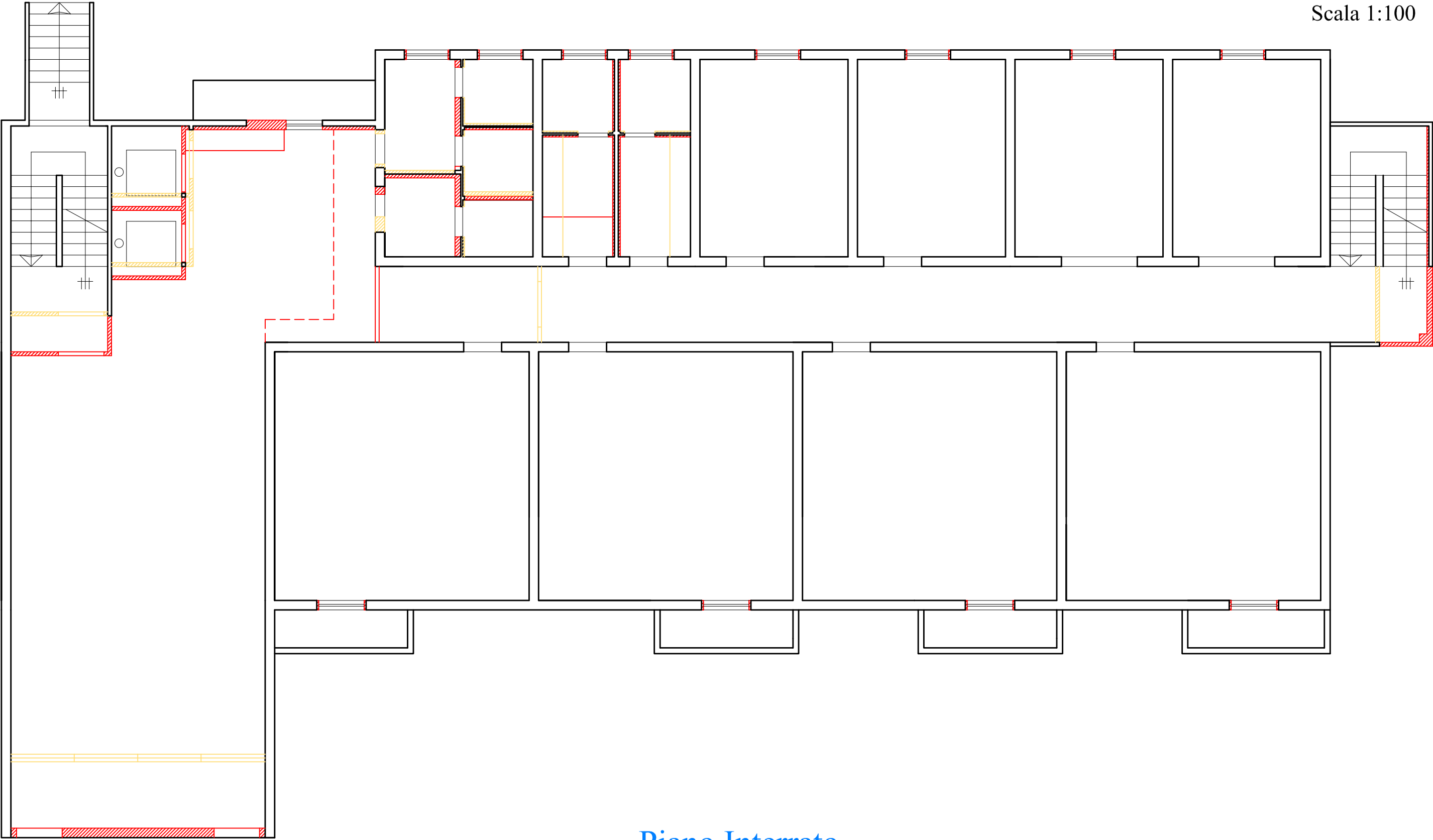
Piano Interrato
